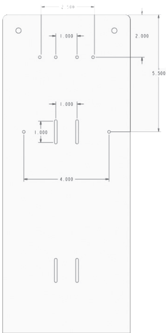
Mounting Specifications
